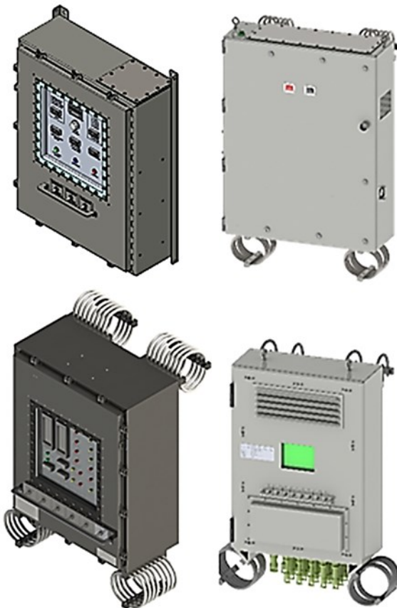
PLC Panels
